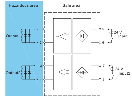
Double input, double output
